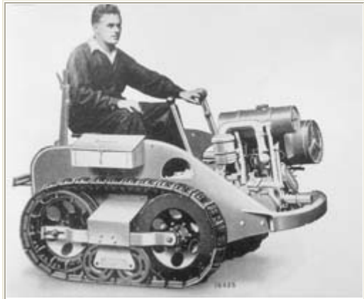
The original Ransomes MG tractor was introduced in 1936 and designated the MG 2. It featured a Sturmev Archer air cooled single cylinder side valve engine developing 6 hp.
